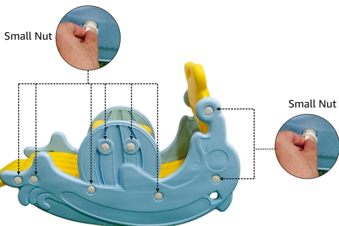
Subassembly (Step 2)
