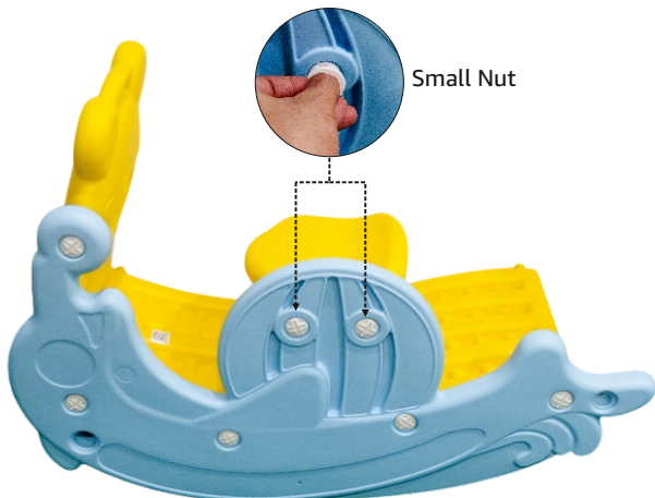
Subassembly (Step 1)
