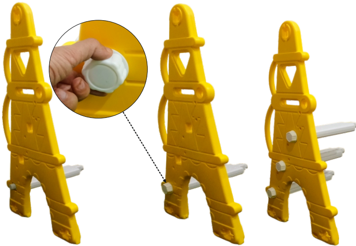
Subassembly (Step 2)
