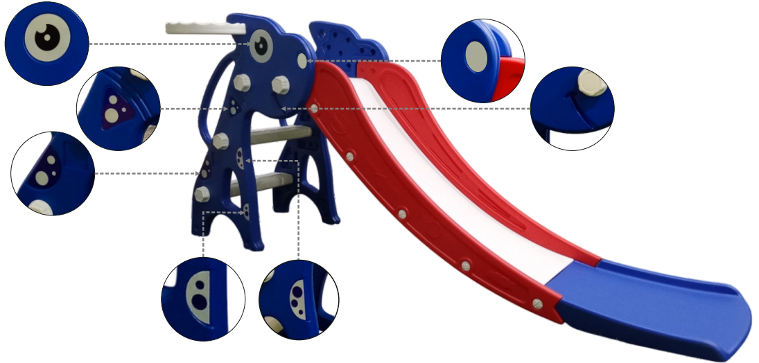
Subassembly (Step 3)
