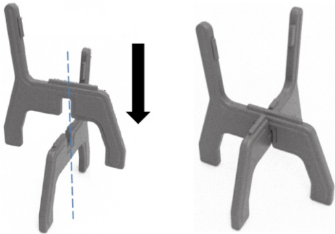
Chair Top Leg x 1
